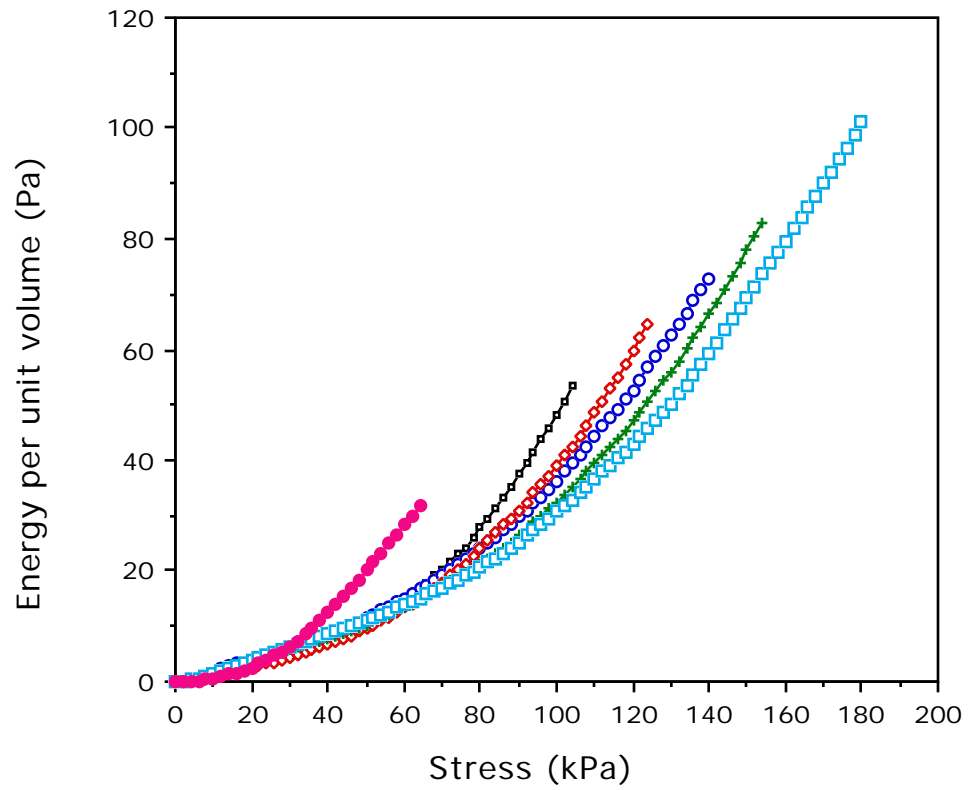
Fig. 11 Energy absorbed per unit volume vs tensile stress for various volumetric compression ratios of Scott industrial foam : • 1.0; , 2.0; , 2.6; , 3.2; + , 3.7; 4.2
