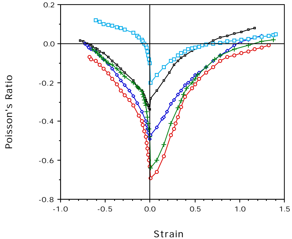
Fig. 6 Poisson's ratio vs strain for Scott industrial foams having different volumetric compression ratios : , 2.0; , 2.6; , 3.2; , 3.7; 4.2
