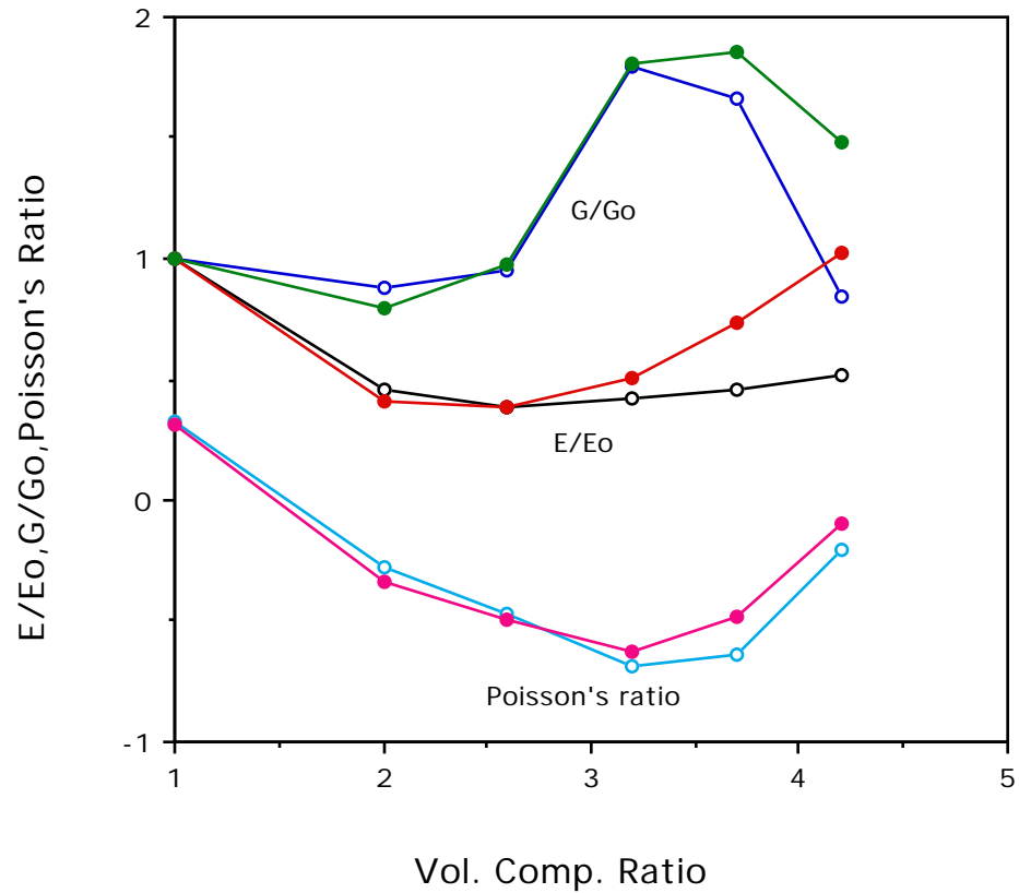
Fig. 12 Measured Young's modulus and Poisson's ratio; calculated shear modulus vs volumetric compression ratio at a strain of 2% in both tension and compression for Scott industrial foam : o , tension; • , compression. E_0 ; 68 kPa in tension, 47 kPa in compression.
