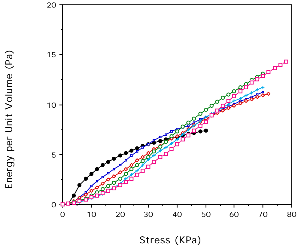
Fig. 10 Energy absorbed per unit volume vs compressive stress for various volumetric compression ratios of Scott industrial foam: •1.0; , 2.0; , 2.6; , 3.2; +, 3.7; 4.2
