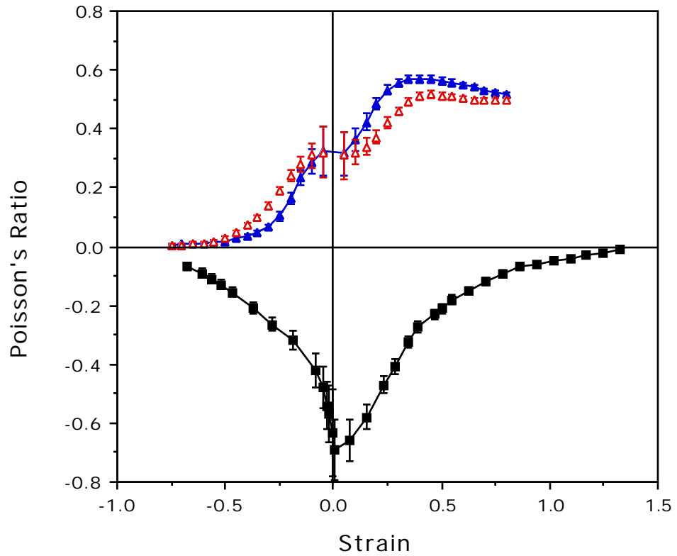
Fig. 2 Poisson's ratio vs longitudinal engineering strain. \blacktriangle : conventional Scott foam; \blacksquare : conventional grey foam; \blacksquare : re-entrant Scott foam with permanent volumetric compression ratio of 3.2.
