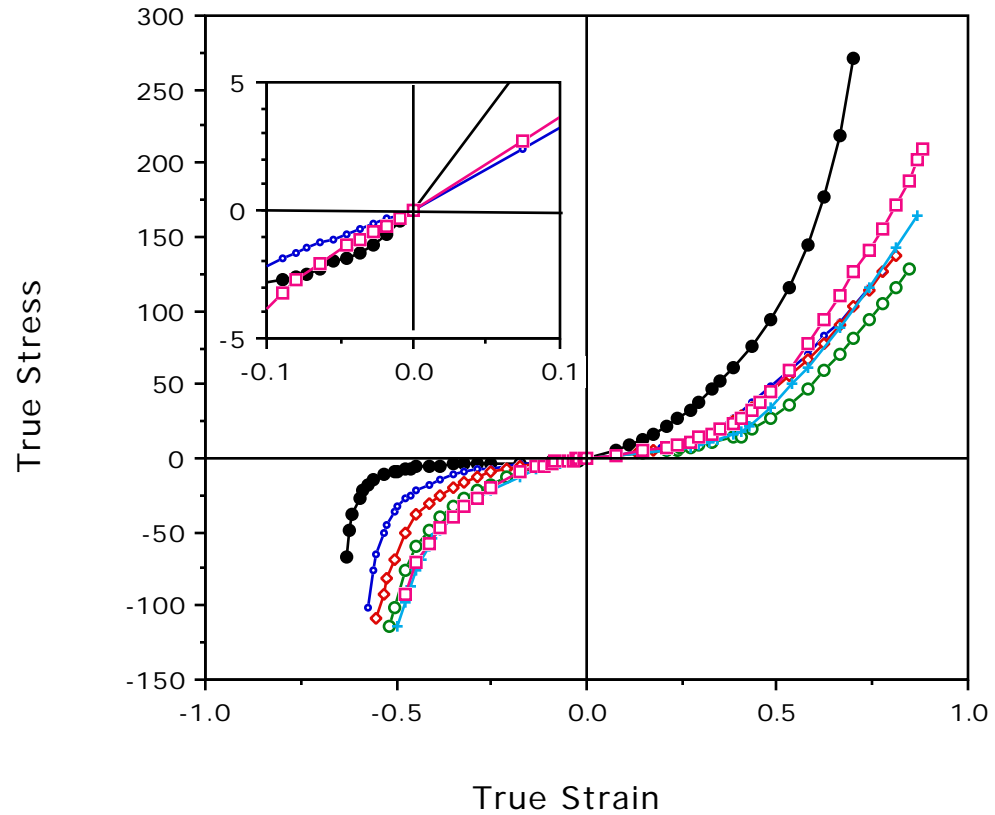
Fig. 8 True stress vs strain for various volumetric compression ratios of Scott industrial foam : •, 1.0; ◊, 2.0; ◻, 2.6; ◊, 3.2; +, 3.7; ◊, 4.2. Inset graph for small strain discloses the compressive nonlinearity of the conventional foam.
