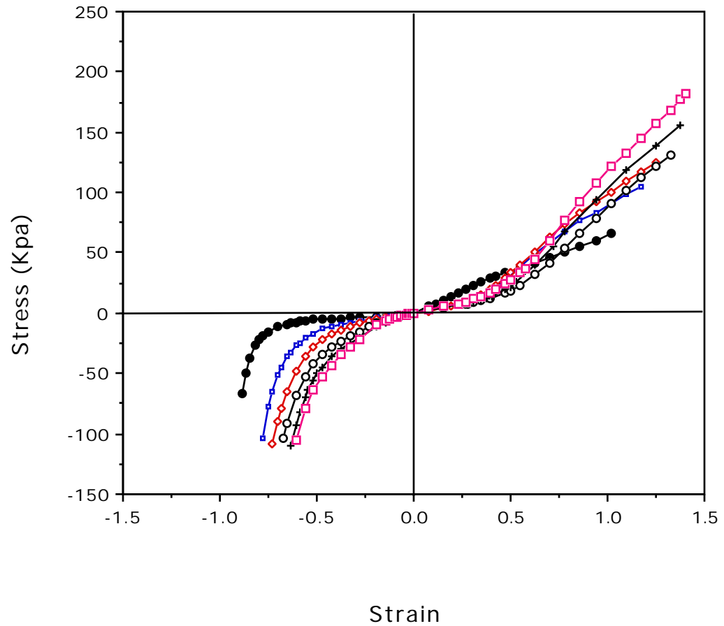
Fig. 7 Engineering stress vs strain for various volumetric compression ratios of Scott industrial foam : •, 1.0; ○, 2.0; □, 2.6; ◇, 3.2; +, 3.7; ×, 4.2.
