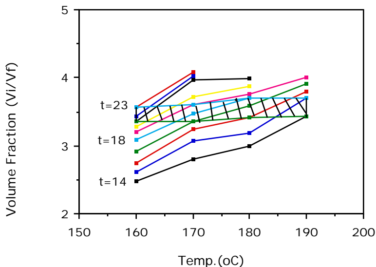
Fig. 1 A plot of volumetric compression ratio vs processing temperature for several processing times t in minutes, for grey polyurethane foam (Shaded region shows the best results for negative Poisson's ratio). Bottom, 14 minutes; top, 23 minutes; 1 min increments. The relative humidity in the laboratory was from 7 to 33%.
