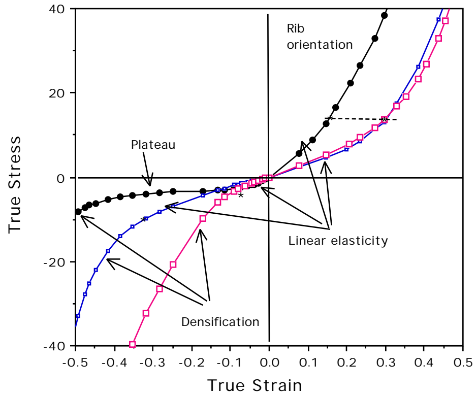
Fig. 9 Deformation mechanism map with stress-strain curves for Scott industrial foam. Regions of linear elasticity, plateau and densification are demarcated by symbol *. Volumetric compression ratios: •, 1.0; □, 2.0; □, 4.2.
