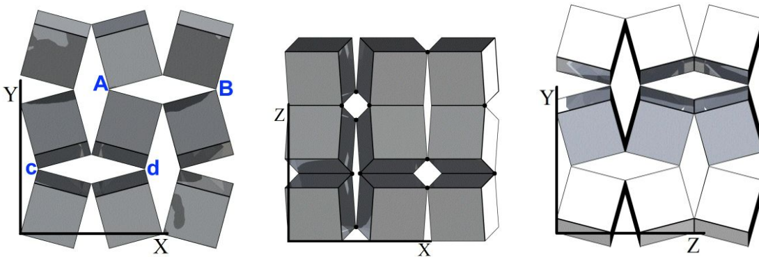
Figure 2: Cube structure, principal direction view.
