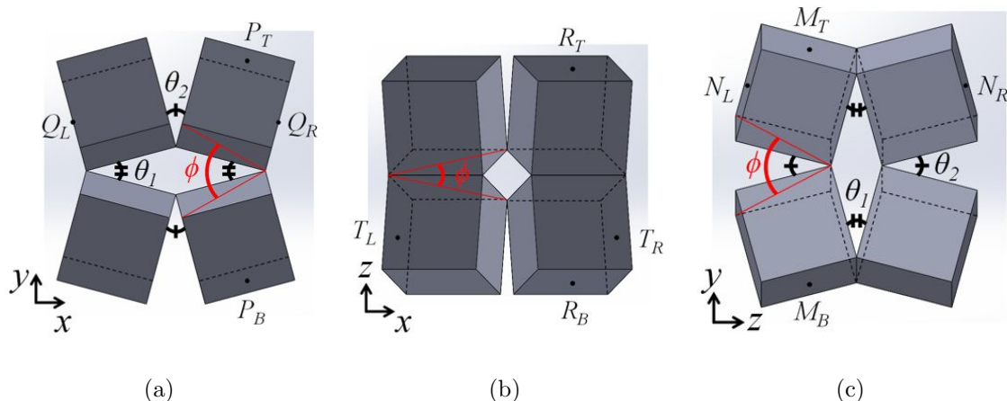
Figure 4: Cube structure viewed along the principal directions. All points are located at the center of cube faces. \phi is an angle between diagonal lines of adjacent cubes. \theta_1 and \theta_2 represent angles between cube edges when the structure is viewed in the corresponding principal directions. For the structure shown, \phi = 42.17^\circ , \theta_1 = 30^\circ and \theta_2 = 28.96^\circ .
