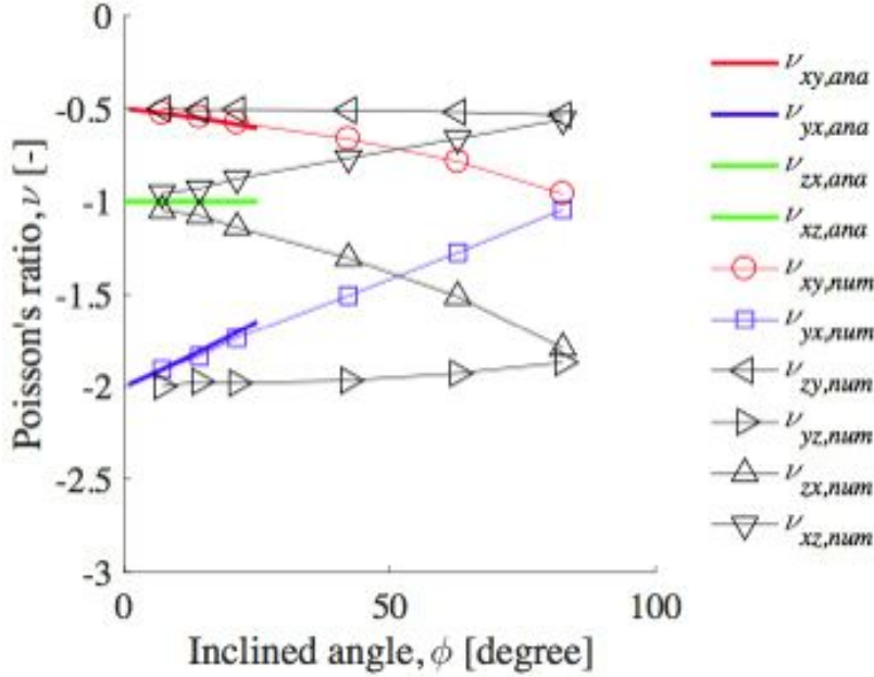
Figure 6: Poisson's ratio in all the principal directions.
