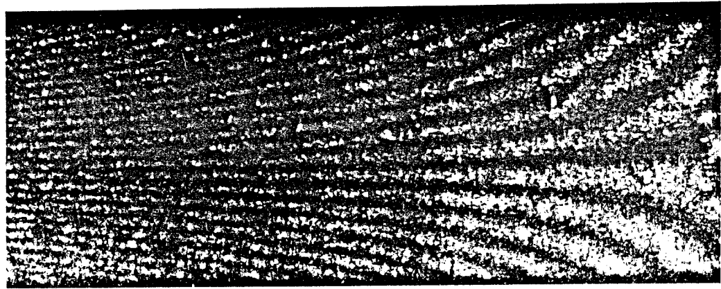
Figure 4 Photograph of a double-exposure hologram of a dense polyurethane foam bar (8.45 mm square cross-section) in torsion. The holographic plate is fixed.
