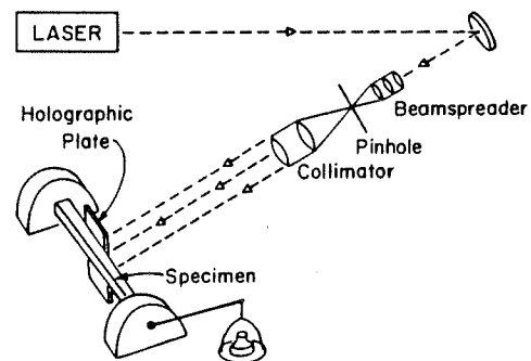
Figure 3 Experimental configuration.
